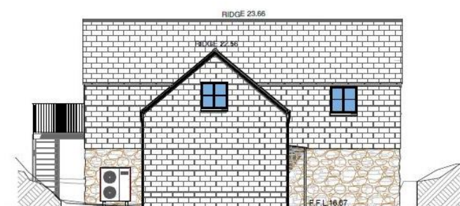
WEST ELEVATION
