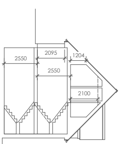
typical section
